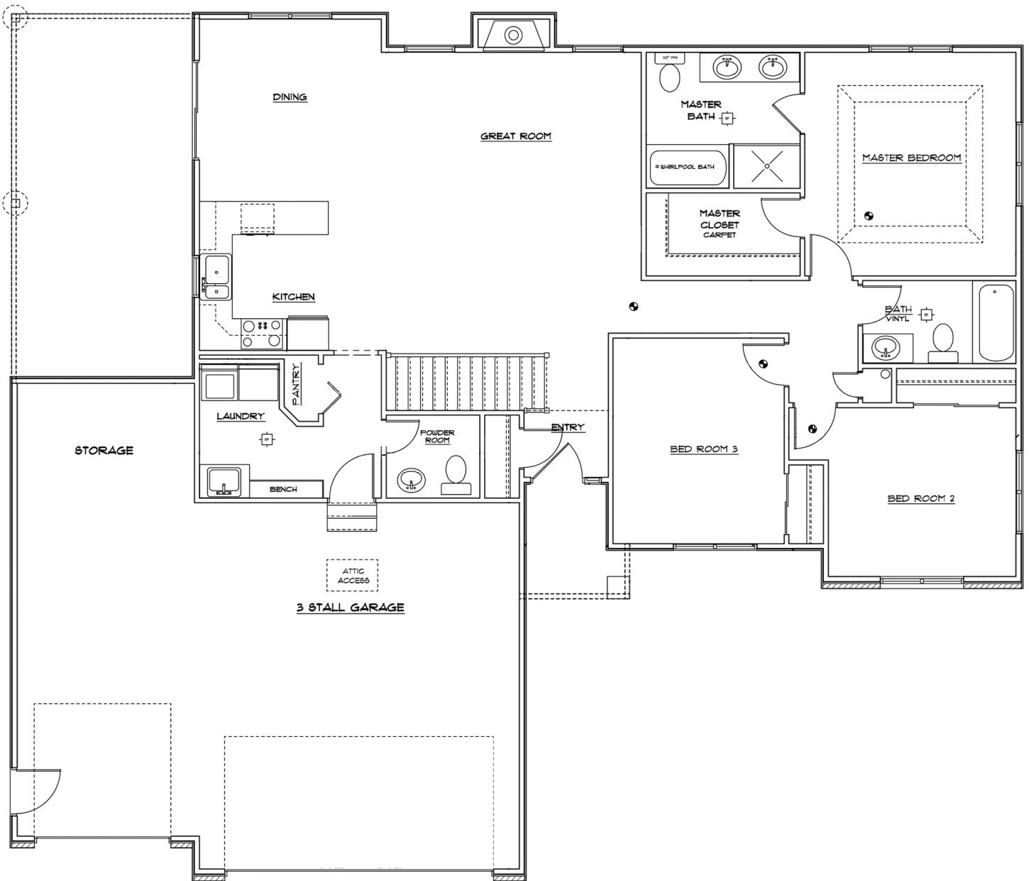
The Richmond: First Floor Plan Sq. Ft. 1514
