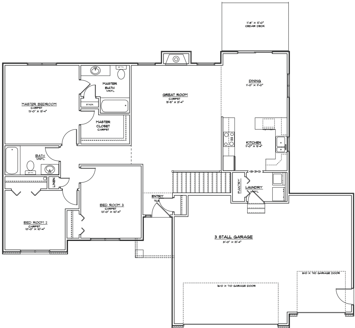
The Oxford: First Floor Plan Sq. Ft. 1387
