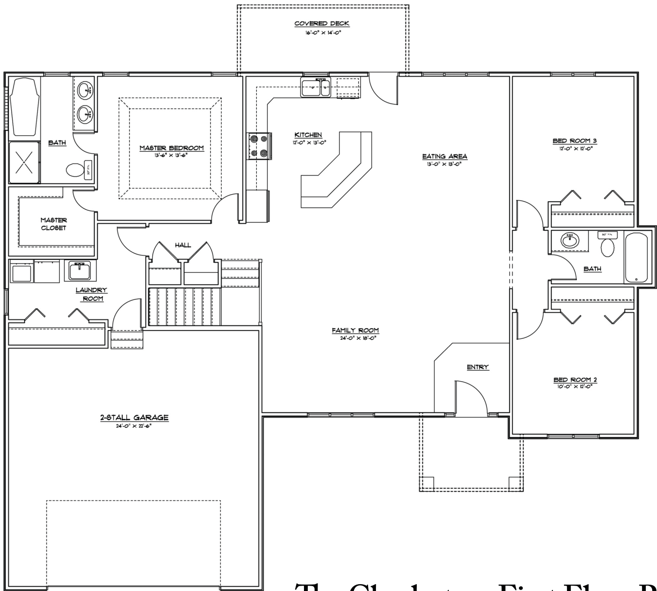
The Charleston: First Floor Plan Sq. Ft. 1745
